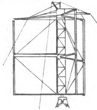
H - DARRIEUS
