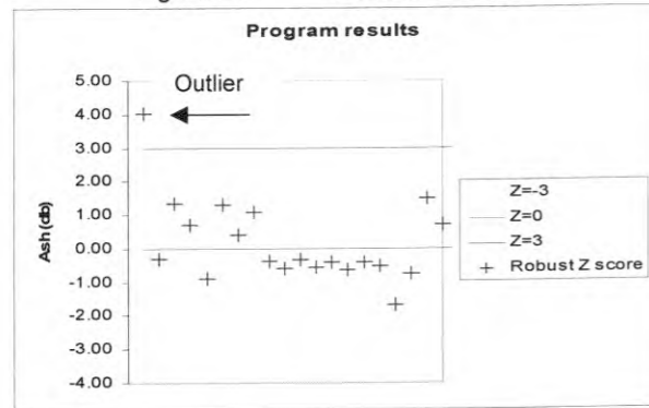
Figure 20. Robust Z Scores
